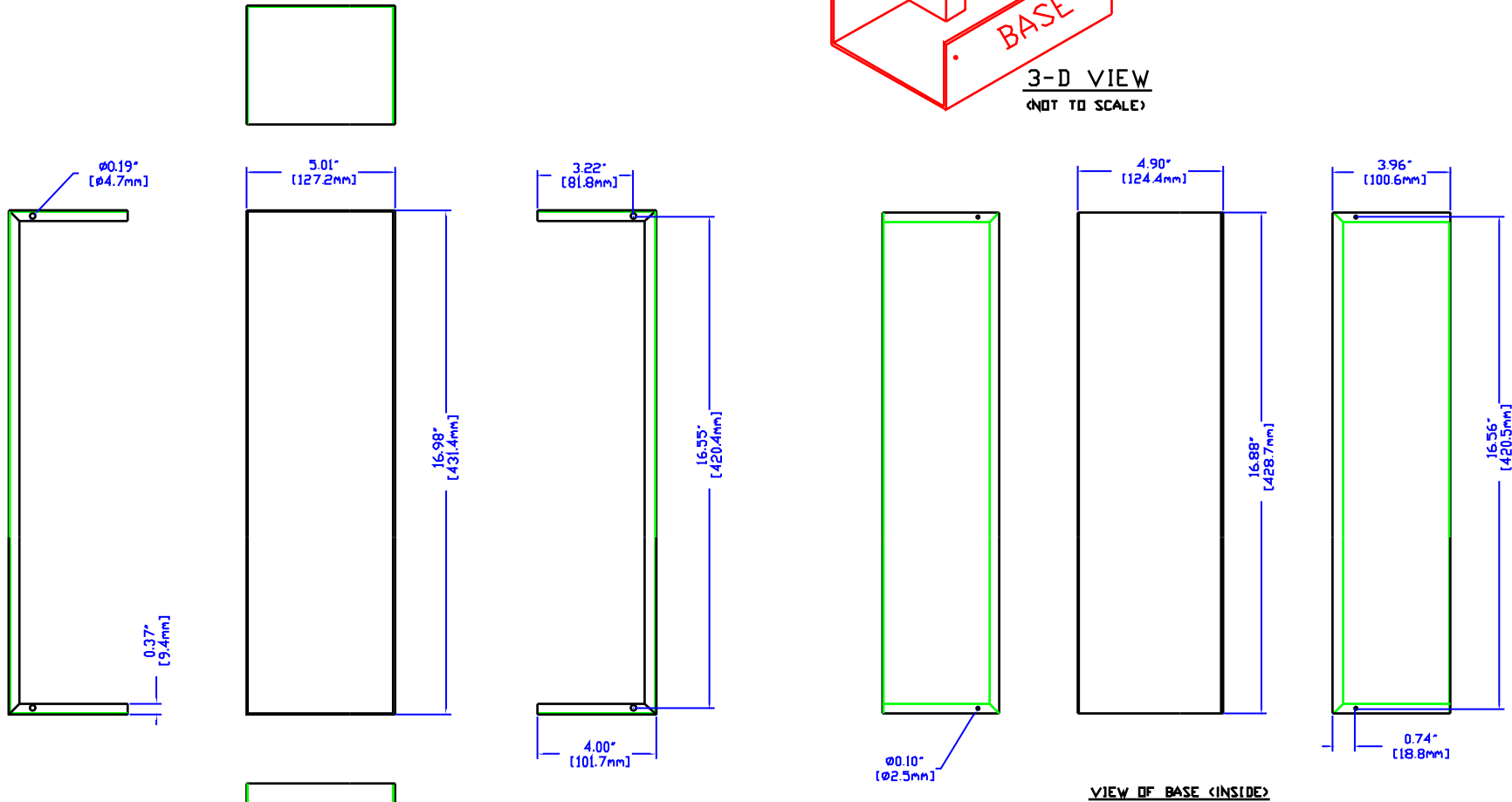
VIEW OF BASE <INSIDE>
